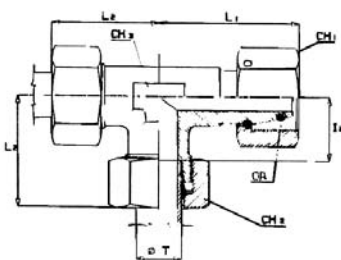
Adjustable male stud T with taper and O-Ring
